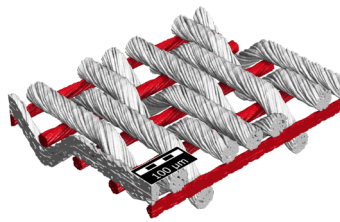
Multifilament reverse Dutch weave
